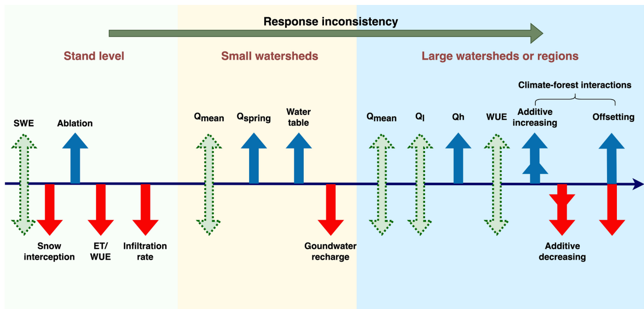
Fig. 1. A visual summary on effects of forest harvesting (or cumulative forest disturbances) on hydrological processes at stand level, small watersheds, and large watersheds or regions (>1000 km 2 ) in boreal forests. Note: WUE, ET, and SWE refer to water use efficiency, evapotranspiration, and snow water equivalent, respectively; Q_{\text{mean}} , Q_{\text{spring}} , Q_i , and Q_h denote annual mean flow, spring flow, low flow, and high flow, respectively.
